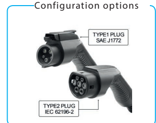
1x or 2x 3 kW - 1x or 2x 44 kW AC charging station
